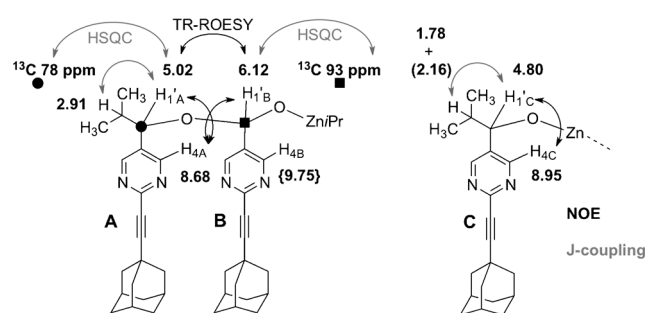
Scheme 2. Observations arising from 2D-NMR spectra of the acetal intermediate 5 at 233 K; the sharp peak at 8.95 ppm does not show relevant cross-peaks but always appears and disappears in concert, as does the broad signal at 9.75 ppm.
